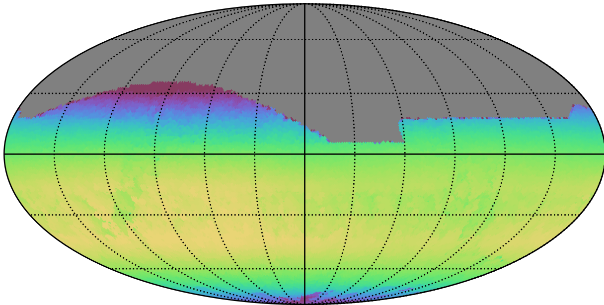
weather_cloudso0v3.4_10yrs All sky z band: Max skyBrightness
