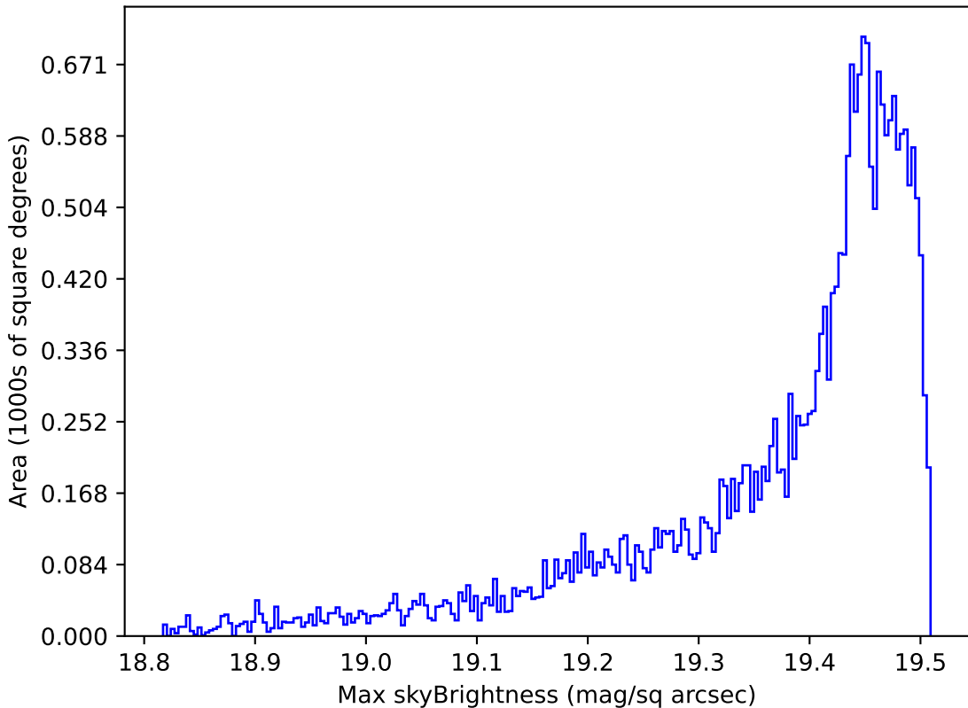
weather_cloudso0v3.4_10yrs All sky z band: Max skyBrightness
