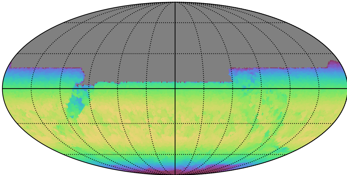
weather_cloudso0v3.4_10yrs All sky y band: Max skyBrightness
