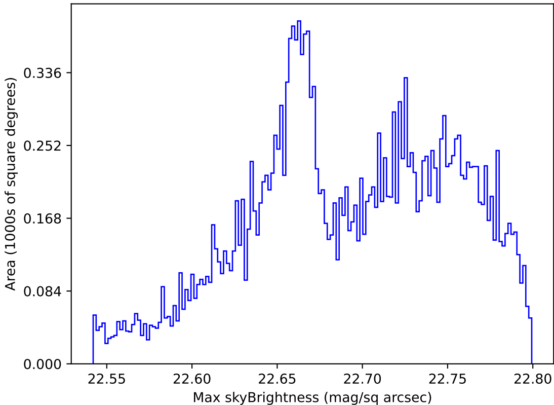
weather_cloudso0v3.4_10yrs All sky u band: Max skyBrightness
