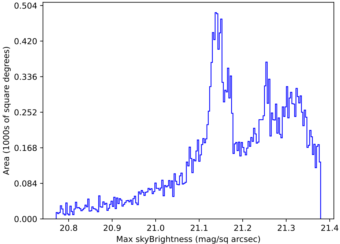
weather_cloudso0v3.4_10yrs All sky r band: Max skyBrightness
