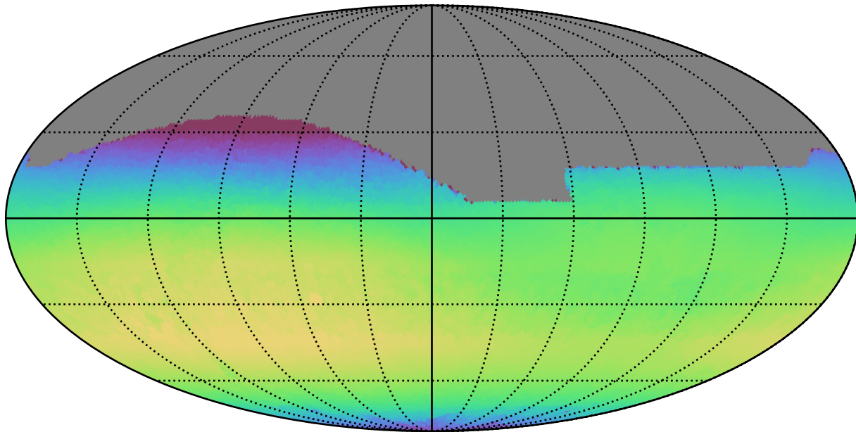
weather_cloudso0v3.4_10yrs All sky i band: Max skyBrightness
