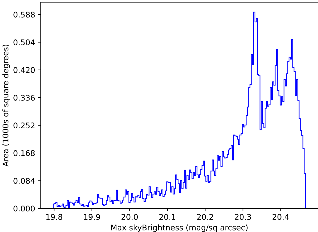
weather_cloudso0v3.4_10yrs All sky i band: Max skyBrightness
