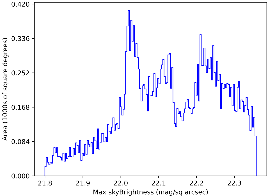
weather_cloudso0v3.4_10yrs All sky g band: Max skyBrightness
