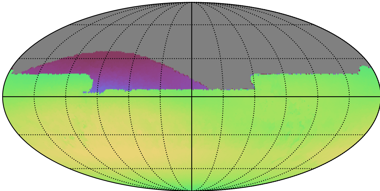
weather_cloudso0v3.4_10yrs All sky all bands: Max skyBrightness
