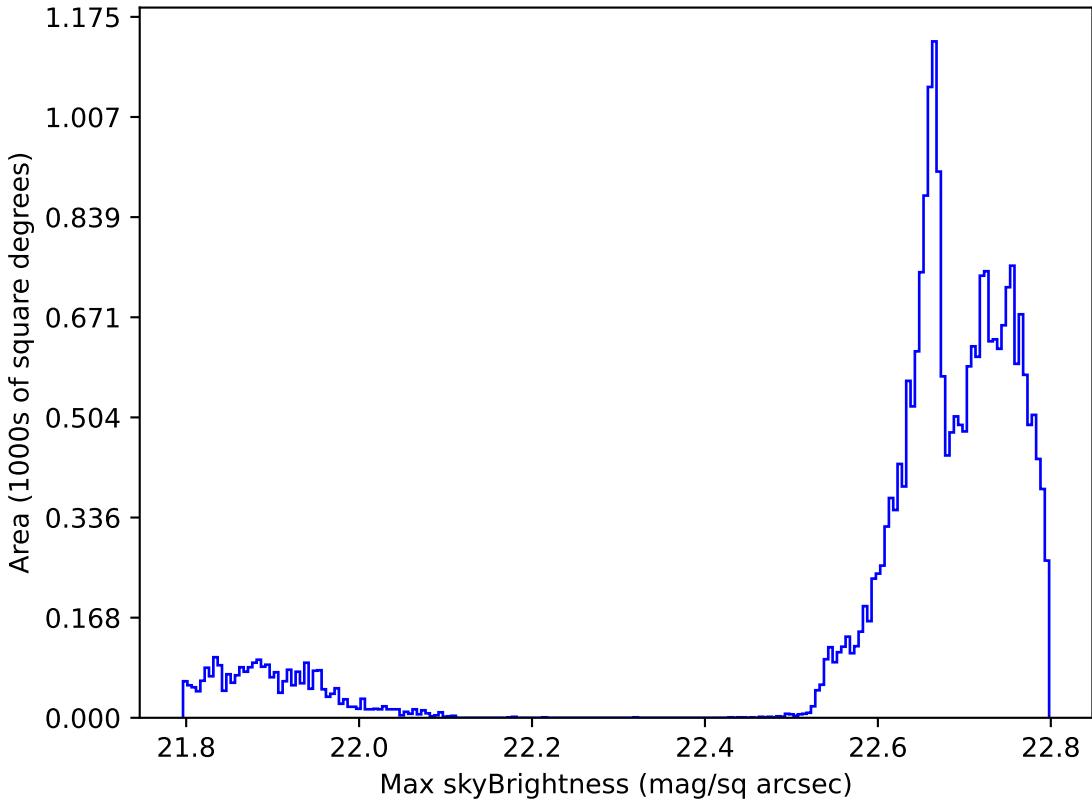
weather_cloudso0v3.4_10yrs All sky all bands: Max skyBrightness
