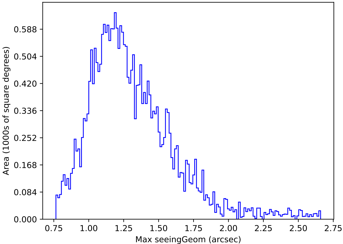
weather_cloudso0v3.4_10yrs Yr 1 z band: Max seeingGeom
