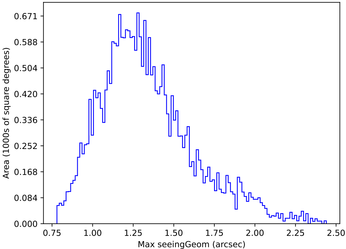
weather_cloudso0v3.4_10yrs Yr 1 r band: Max seeingGeom
