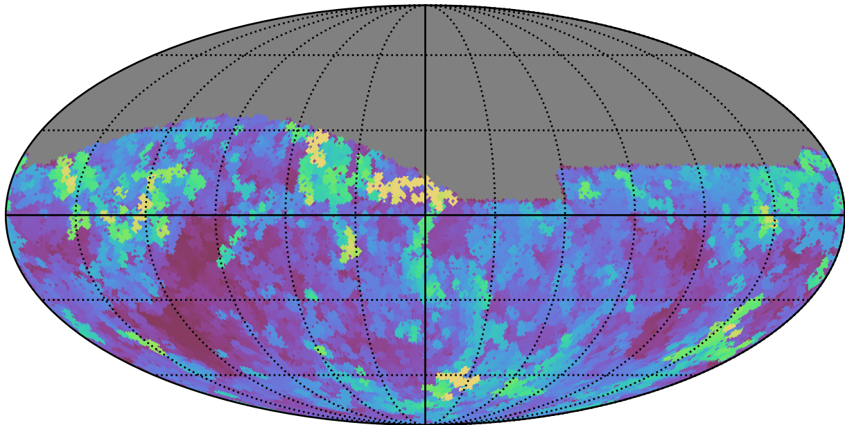
weather_cloudso0v3.4_10yrs Yr 1 i band: Max seeingGeom
