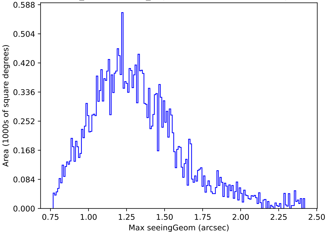
weather_cloudso0v3.4_10yrs Yr 1 i band: Max seeingGeom
