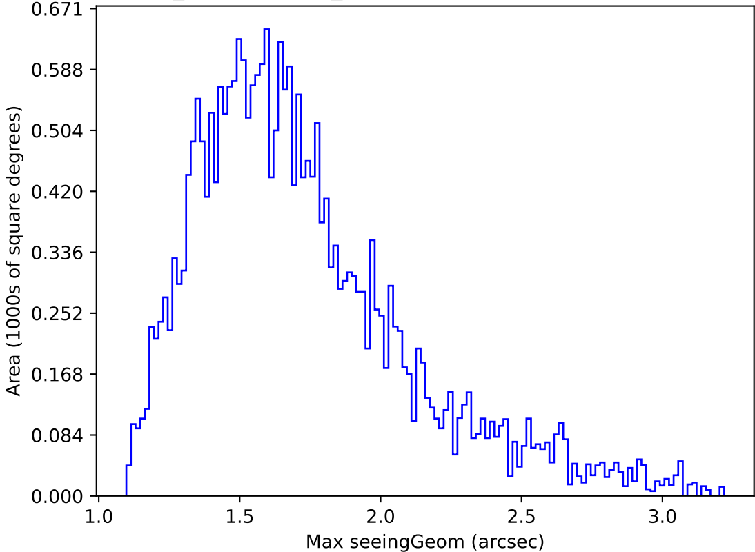
weather_cloudso0v3.4_10yrs Yr 1 all bands: Max seeingGeom
