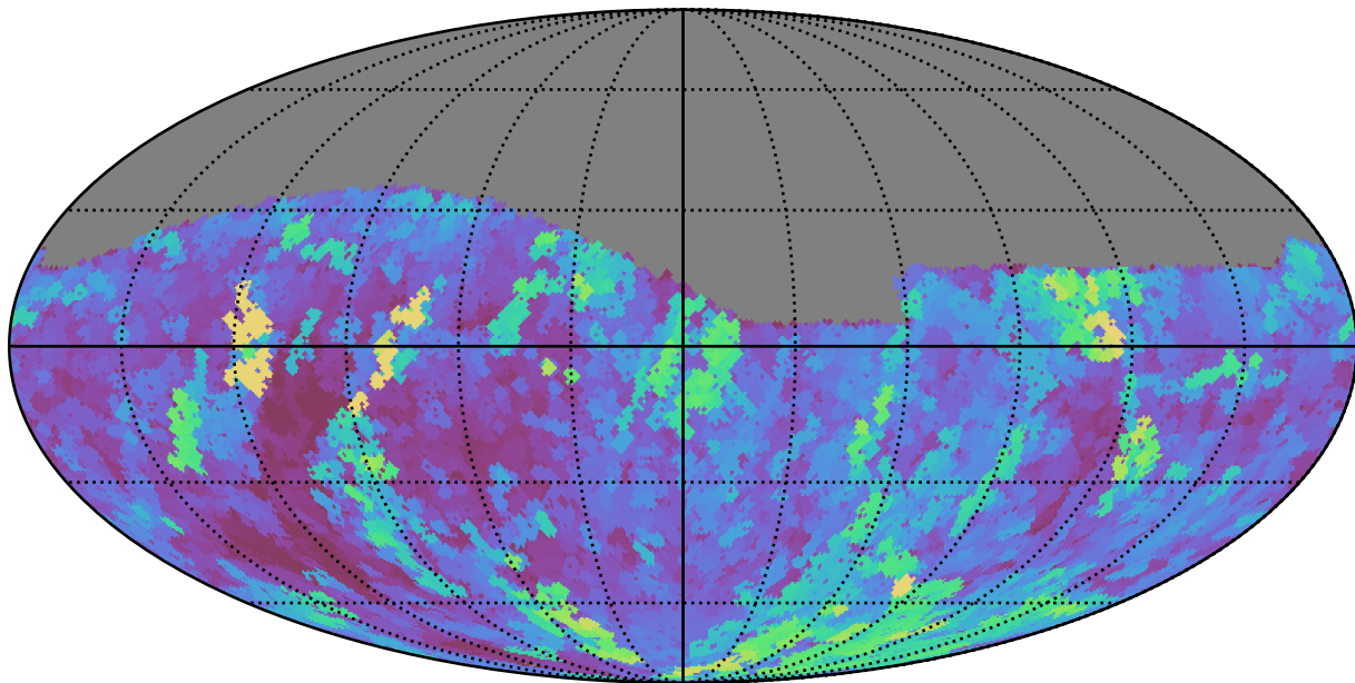
weather_cloudso0v3.4_10yrs Yr 1 r band: Max seeingEff
