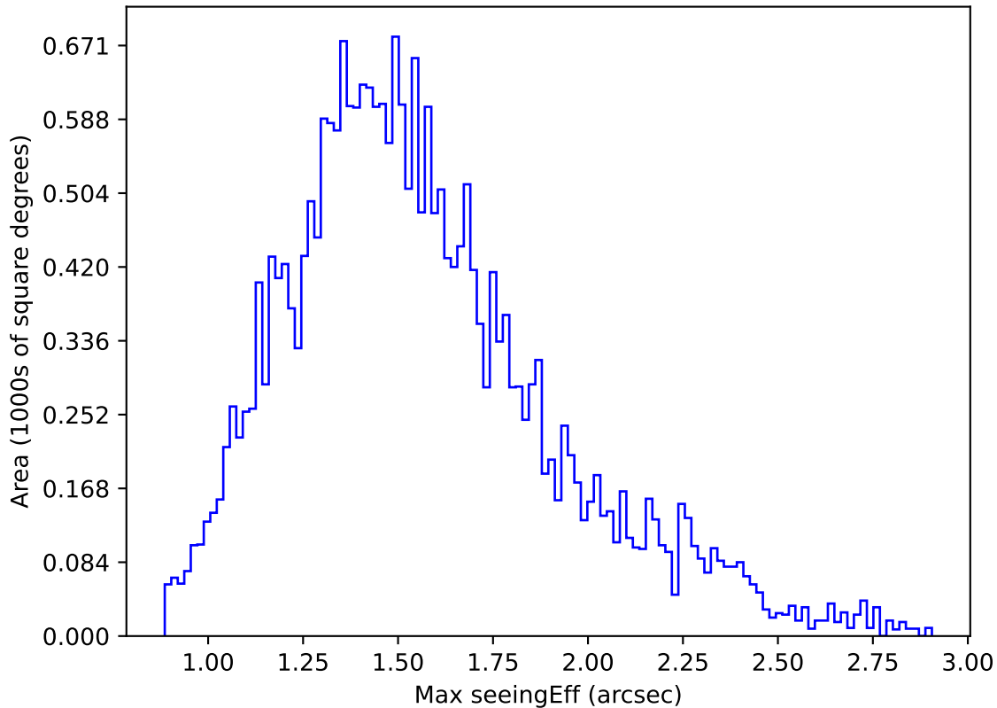
weather_cloudso0v3.4_10yrs Yr 1 r band: Max seeingEff
