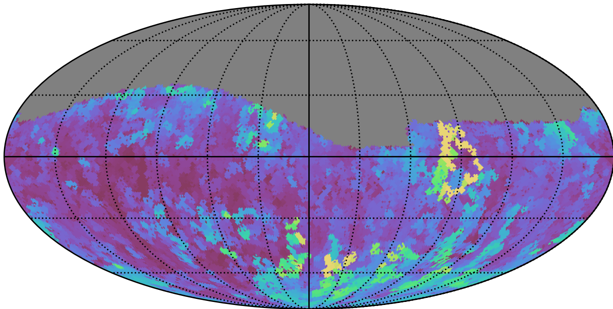
weather_cloudso0v3.4_10yrs Yr 1 g band: Max seeingEff
