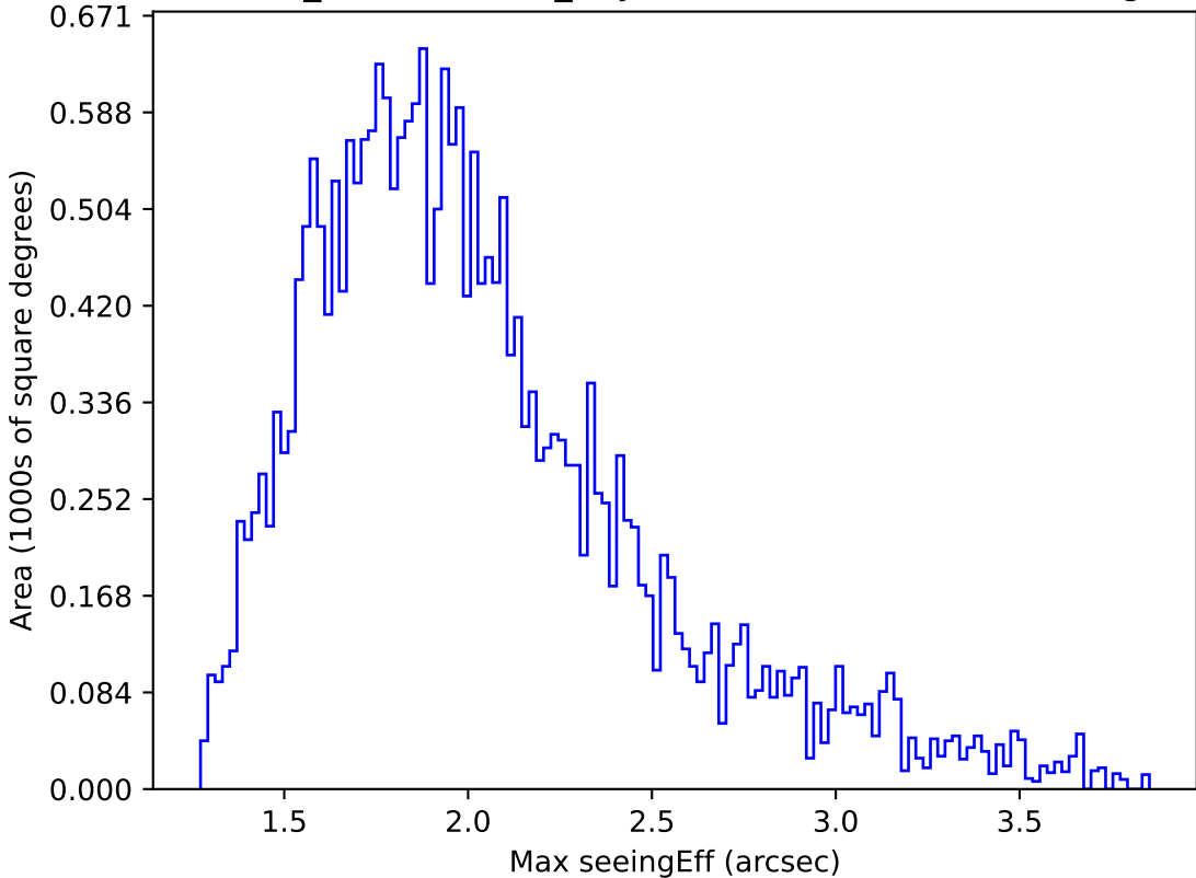
weather_cloudso0v3.4_10yrs Yr 1 all bands: Max seeingEff
