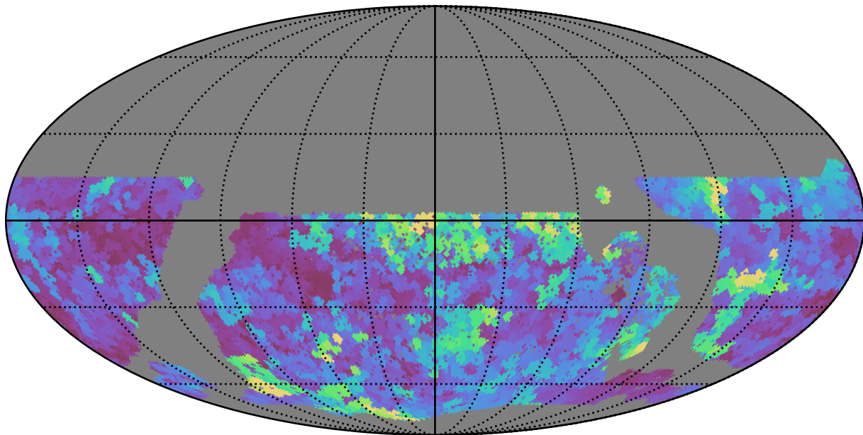
weather_cloudso0v3.4_10yrs WFD u band: Max seeingEff
