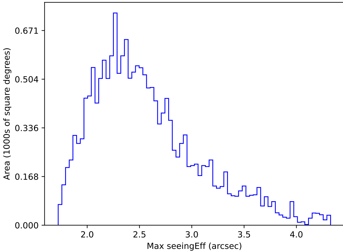
weather_cloudso0v3.4_10yrs WFD u band: Max seeingEff
