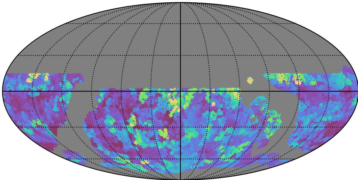
weather_cloudso0v3.4_10yrs WFD r band: Max seeingEff
