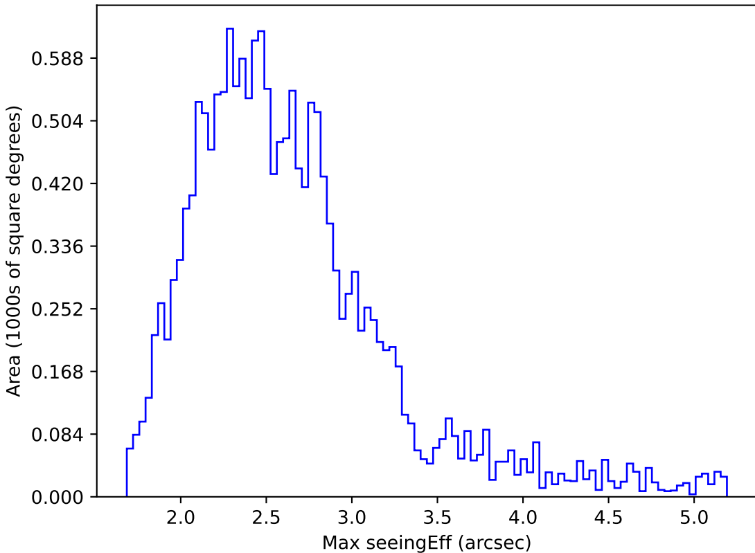
weather_cloudso0v3.4_10yrs WFD i band: Max seeingEff
