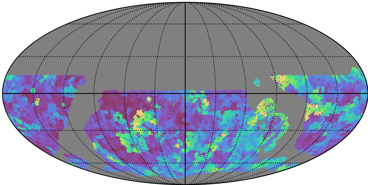
weather_cloudso0v3.4_10yrs WFD g band: Max seeingEff
