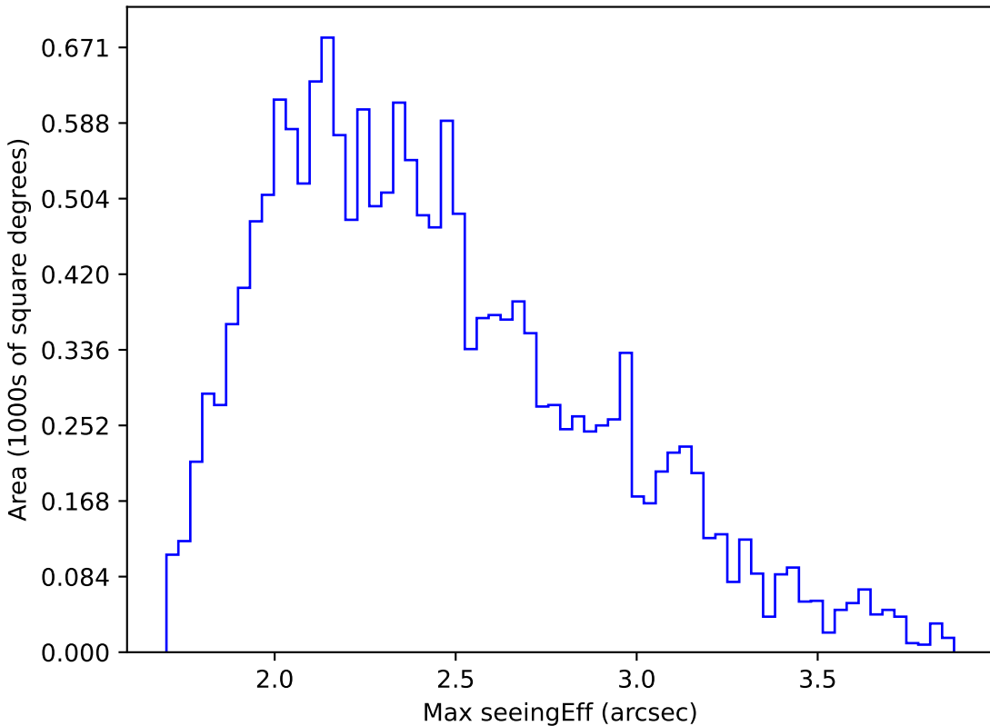
weather_cloudso0v3.4_10yrs WFD g band: Max seeingEff
