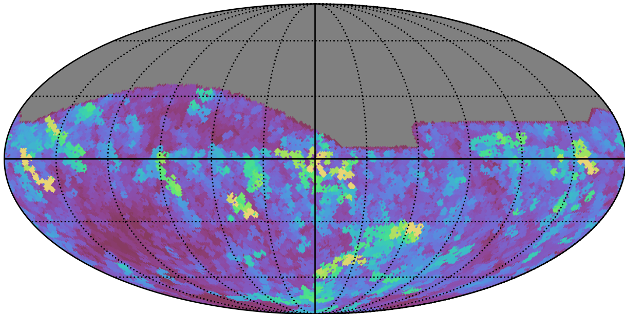
weather_cloudso0v3.4_10yrs All sky z band: Max seeingEff
