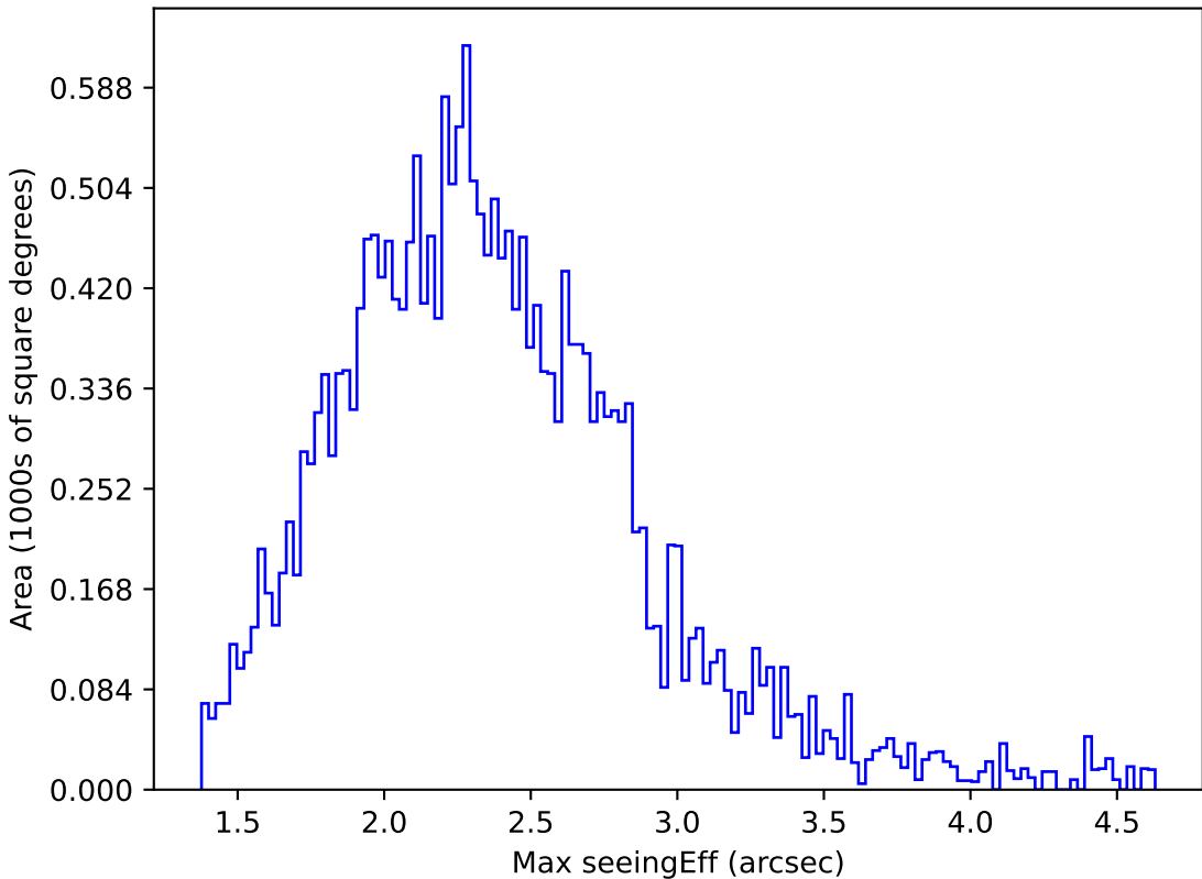
weather_cloudso0v3.4_10yrs All sky y band: Max seeingEff
