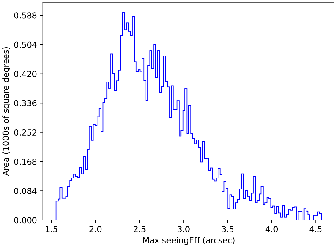
weather_cloudso0v3.4_10yrs All sky r band: Max seeingEff
