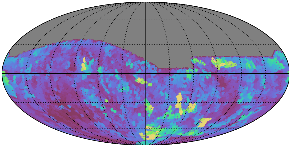
weather_cloudso0v3.4_10yrs All sky i band: Max seeingEff
