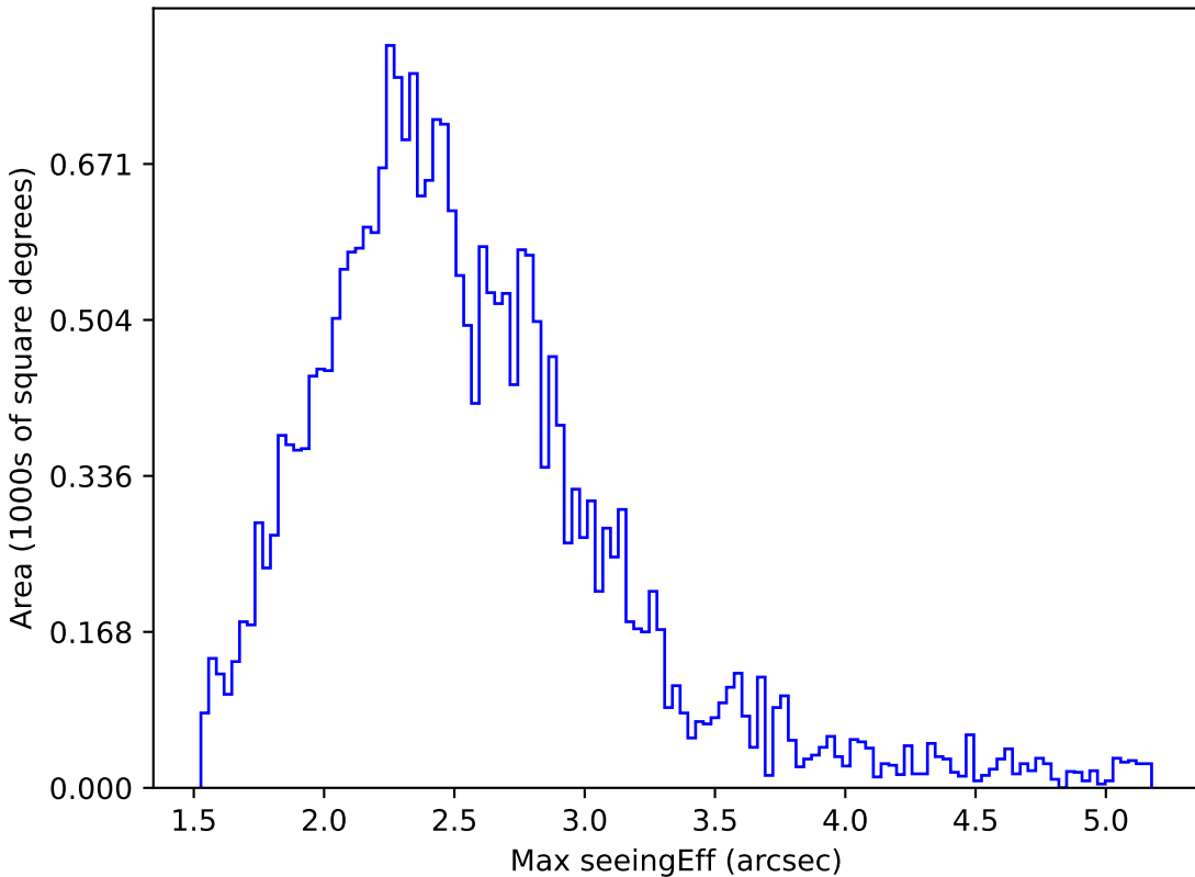
weather_cloudso0v3.4_10yrs All sky i band: Max seeingEff
