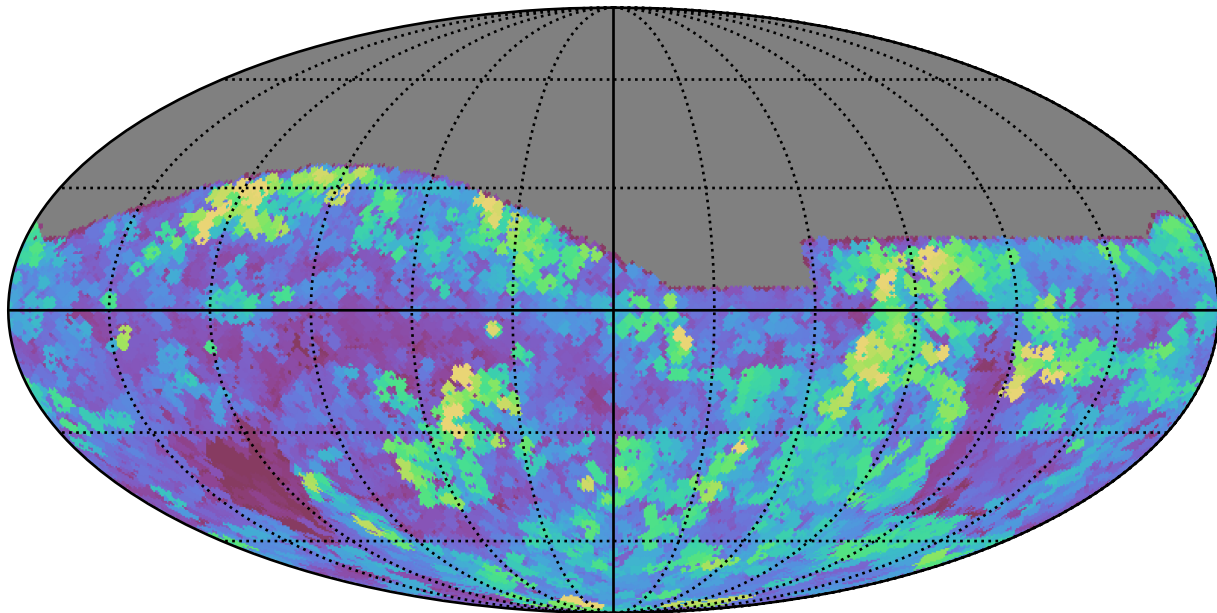
weather_cloudso0v3.4_10yrs All sky g band: Max seeingEff
