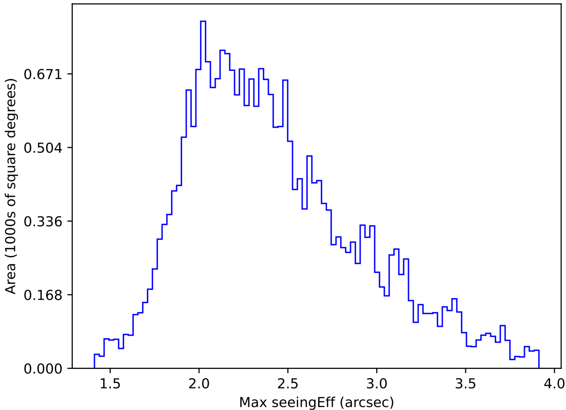
weather_cloudso0v3.4_10yrs All sky g band: Max seeingEff
