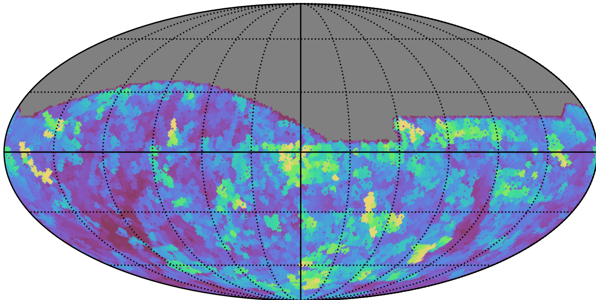
weather_cloudso0v3.4_10yrs All sky all bands: Max seeingEff
