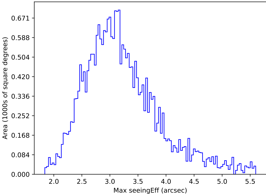
weather_cloudso0v3.4_10yrs All sky all bands: Max seeingEff
