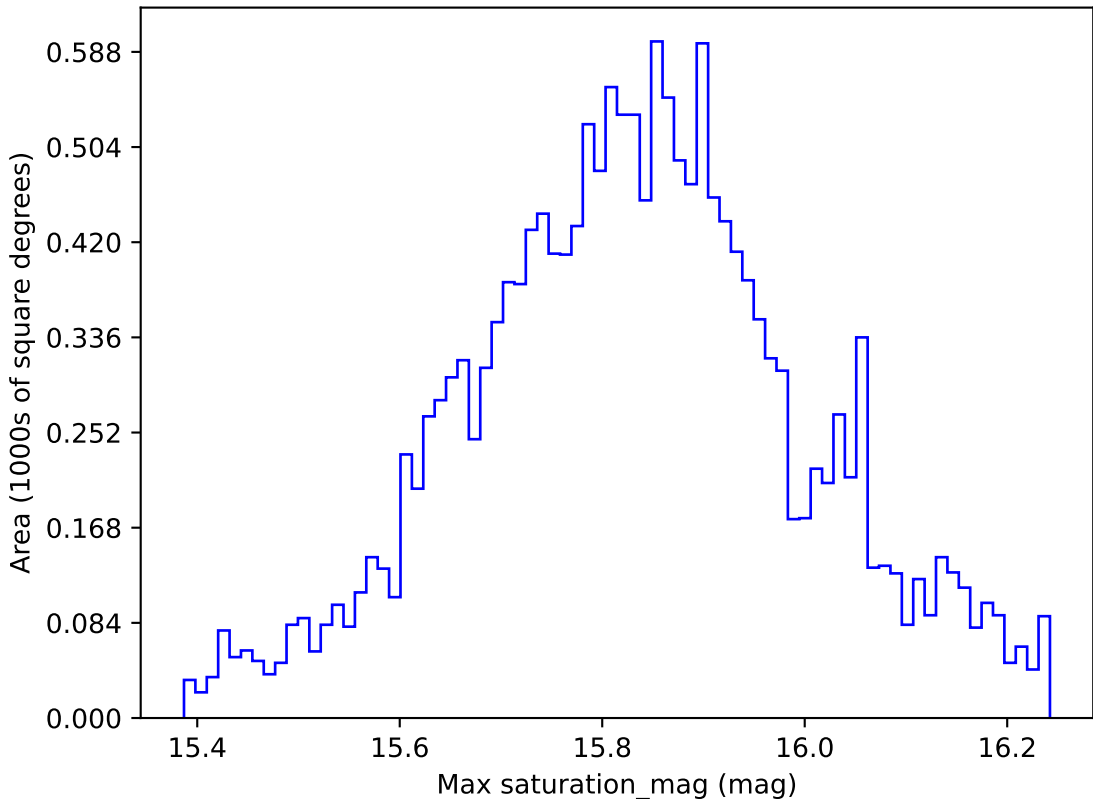
weather_cloudso0v3.4_10yrs WFD all bands: Max saturation_mag
