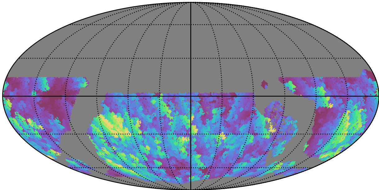
weather_cloudso0v3.4_10yrs WFD u band: Max normairmass
