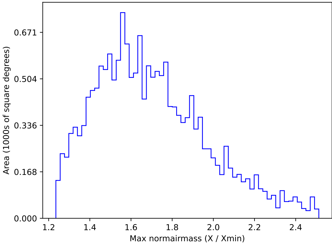
weather_cloudso0v3.4_10yrs WFD u band: Max normairmass
