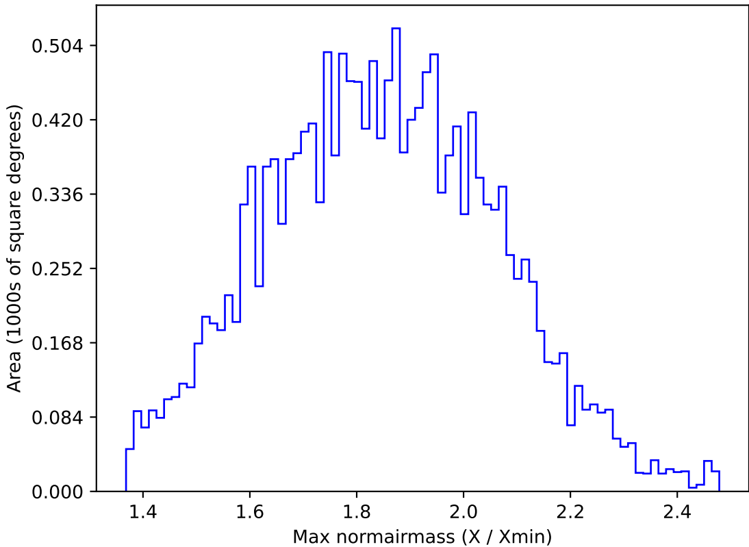
weather_cloudso0v3.4_10yrs WFD g band: Max normairmass
