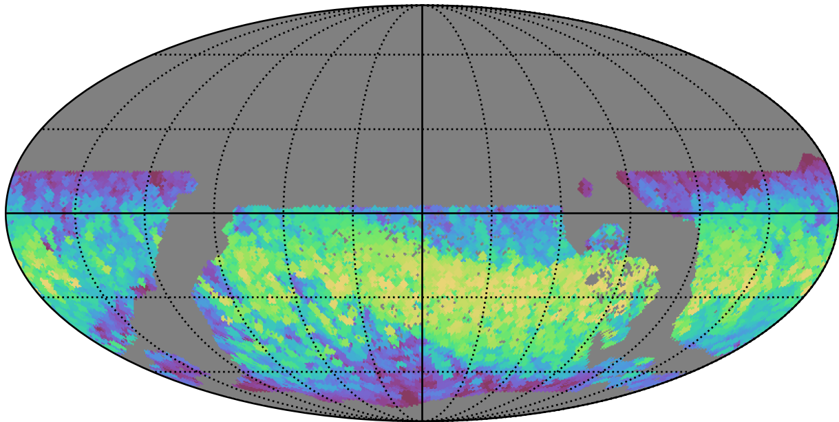
weather_cloudso0v3.4_10yrs WFD all bands: Max normairmass
