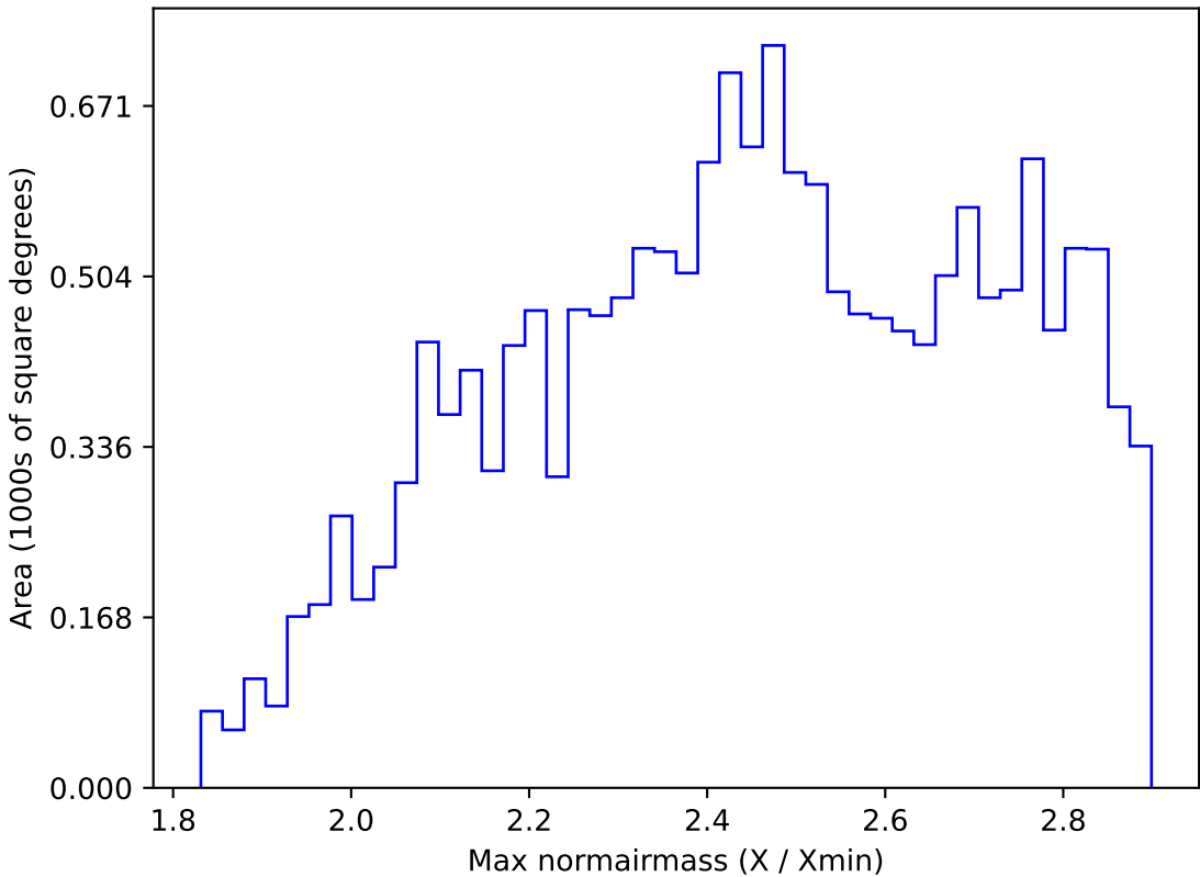
weather_cloudso0v3.4_10yrs WFD all bands: Max normairmass
