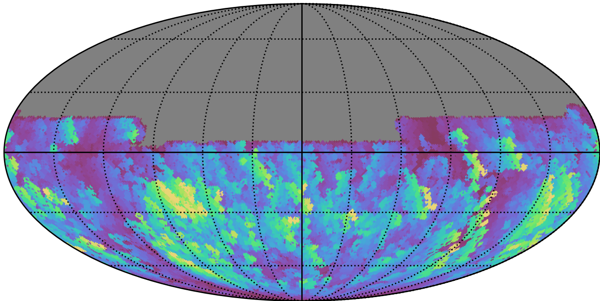
weather_cloudso0v3.4_10yrs All sky u band: Max normairmass
