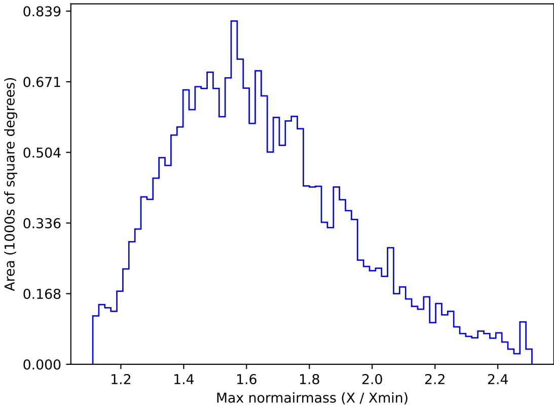
weather_cloudso0v3.4_10yrs All sky u band: Max normairmass
