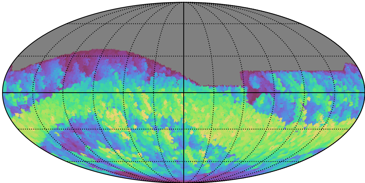
weather_cloudso0v3.4_10yrs All sky r band: Max normairmass
