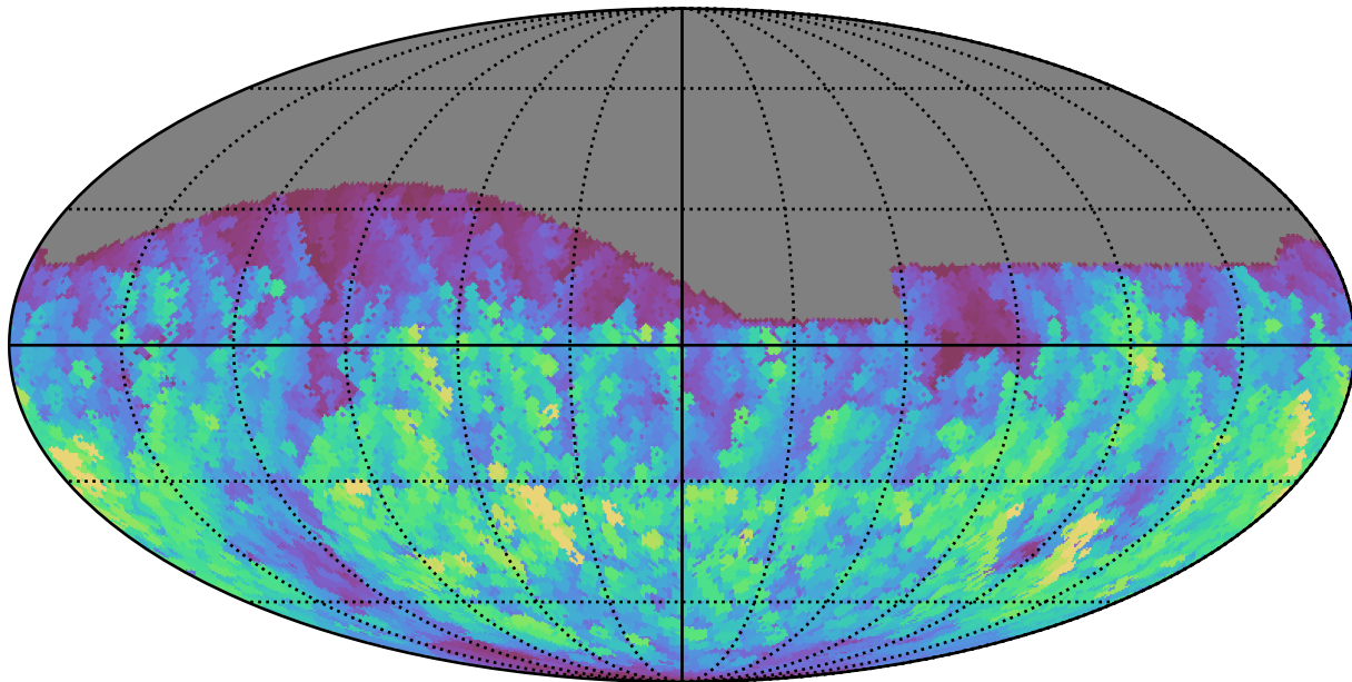
weather_cloudso0v3.4_10yrs All sky g band: Max normairmass
