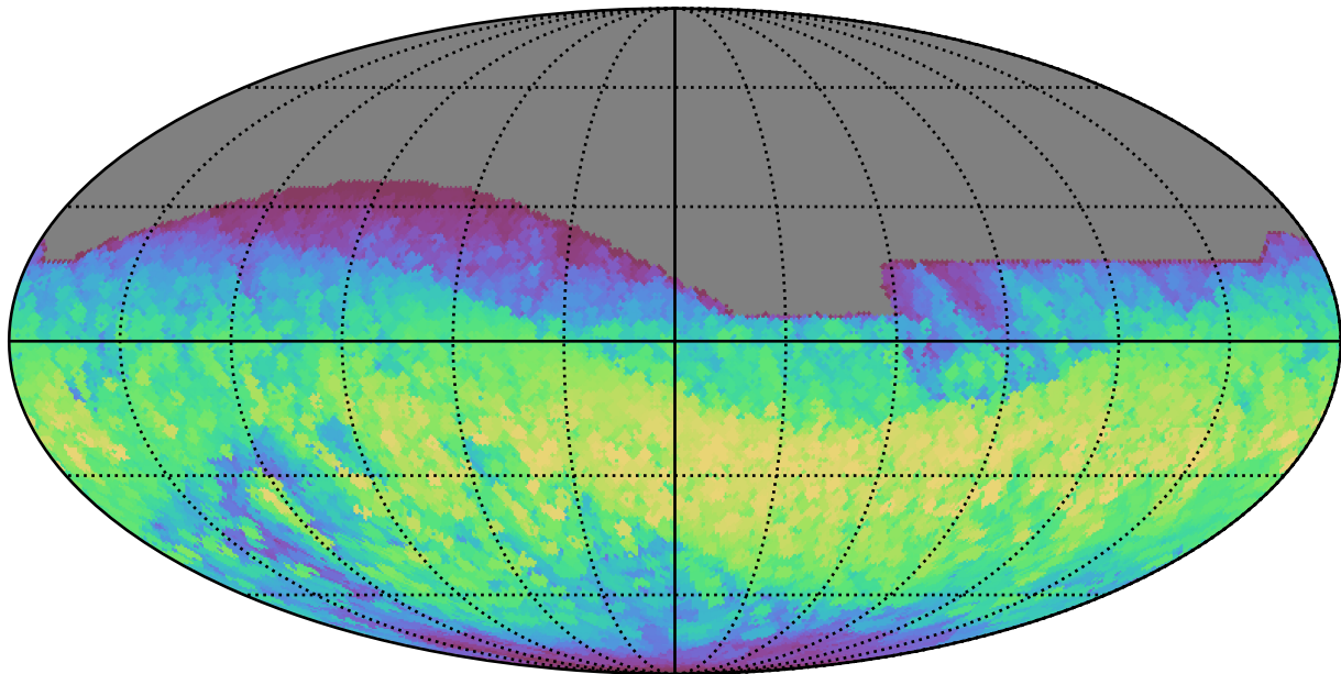
weather_cloudso0v3.4_10yrs All sky all bands: Max normairmass
