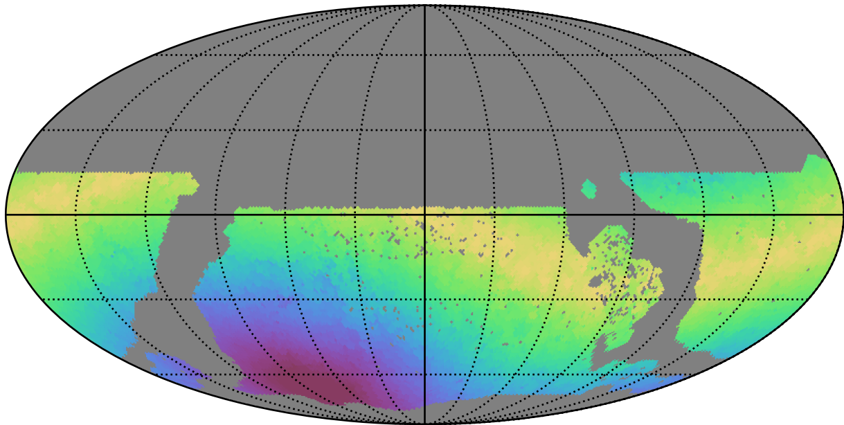
weather_cloudso0v3.4_10yrs WFD z band: Max moonDistance
