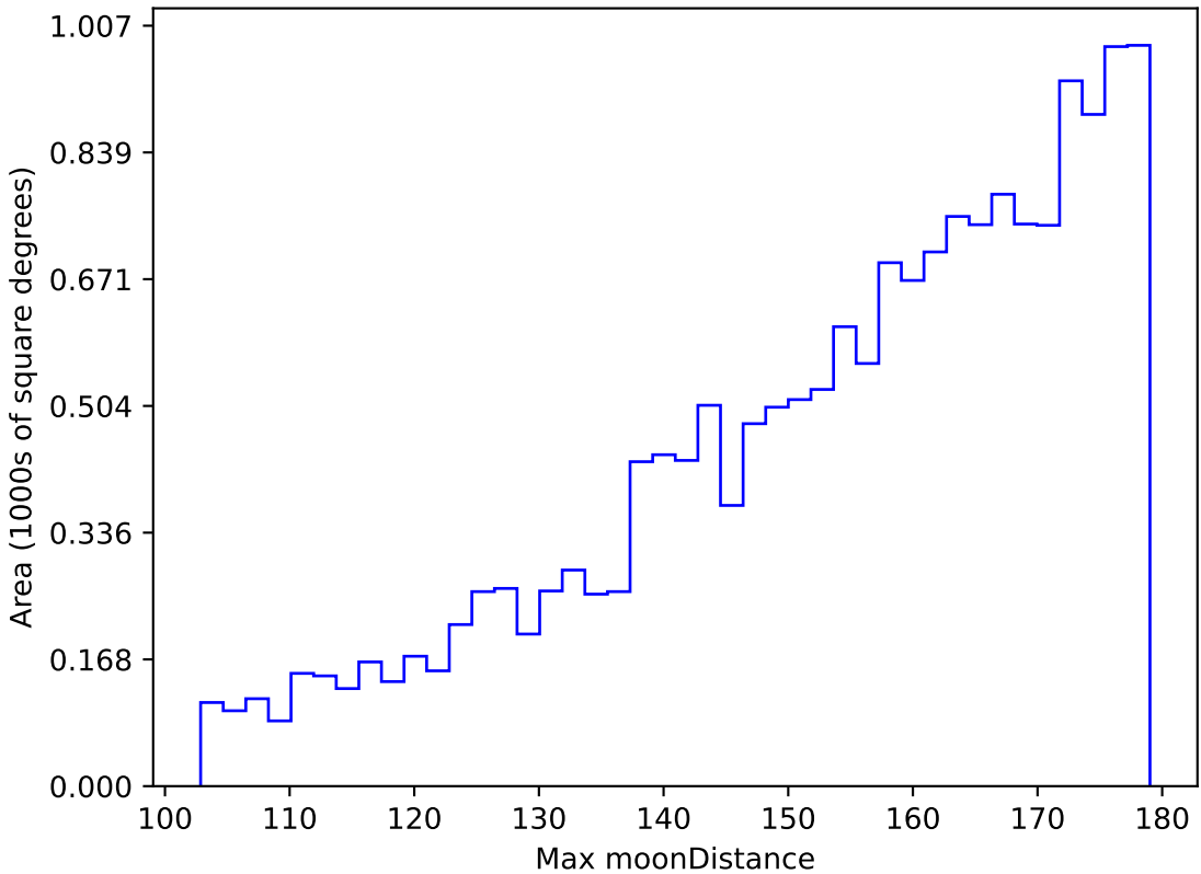
weather_cloudso0v3.4_10yrs WFD z band: Max moonDistance
