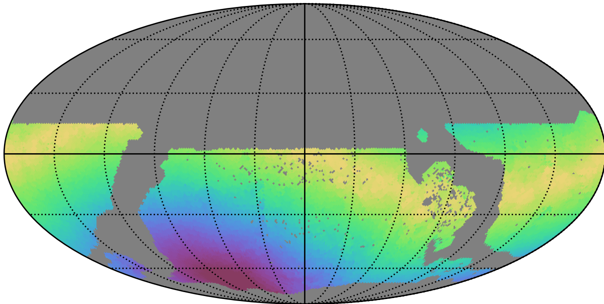
weather_cloudso0v3.4_10yrs WFD u band: Max moonDistance
