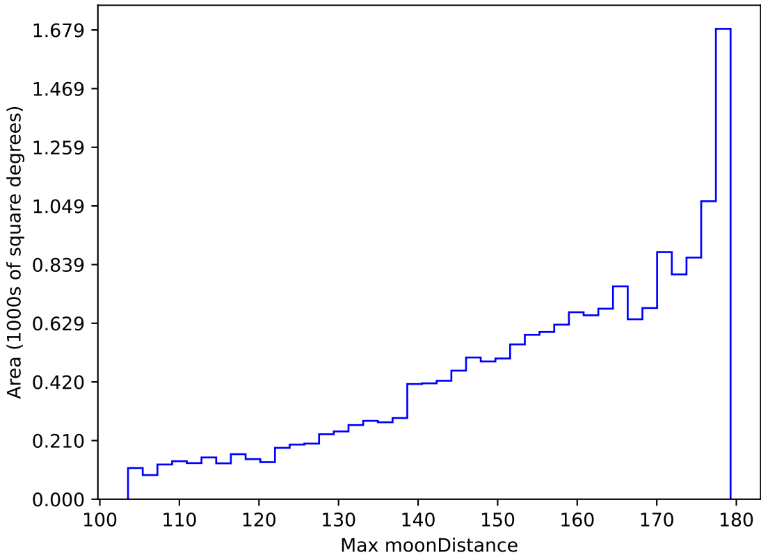
weather_cloudso0v3.4_10yrs WFD r band: Max moonDistance
