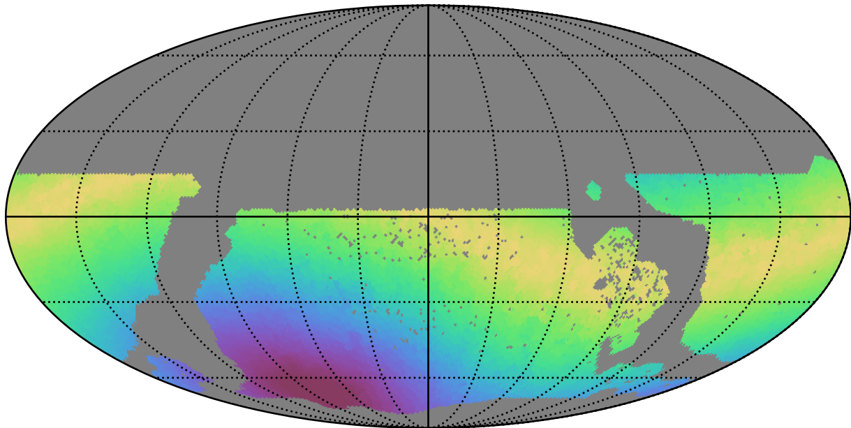
weather_cloudso0v3.4_10yrs WFD i band: Max moonDistance
